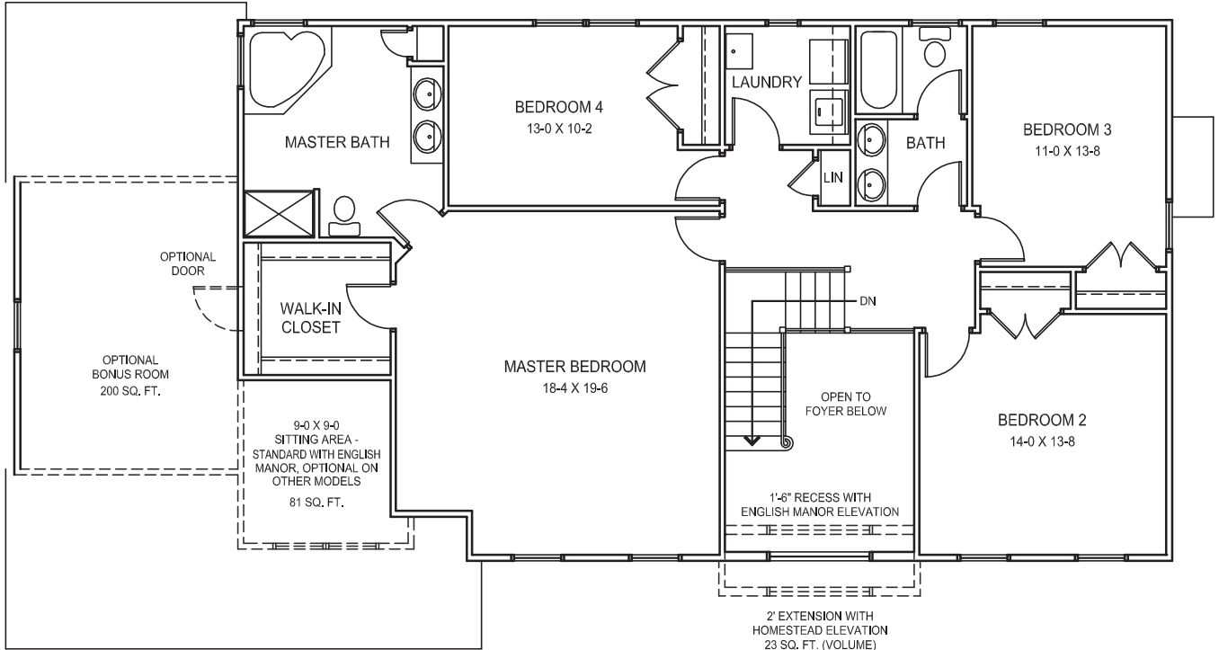
1364 - SECOND FLOOR
